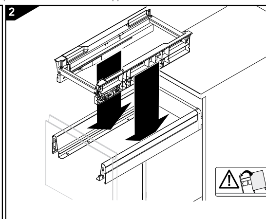
Place bin frame over drawer
