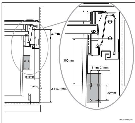
Blum TANDEMBOX drawer front drilling position & 560 additional support brackets
