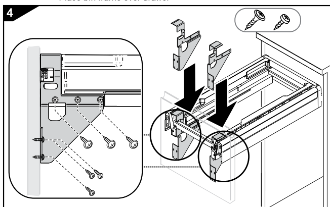
Assemble support bracket
