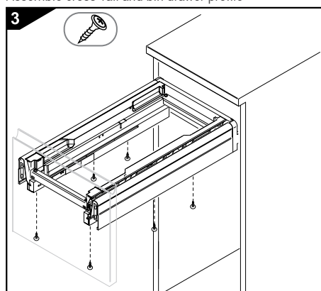
Fix bin frame to drawer
