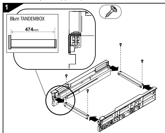
Assemble cross-rail and bin drawer profile
