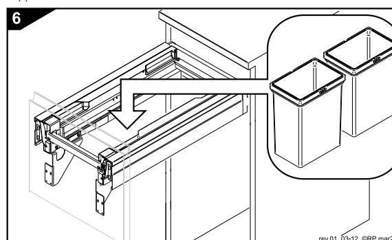
Place buckets into frame; Ready for front panel assembly; Screw off support brackets after final adjustments on site.
